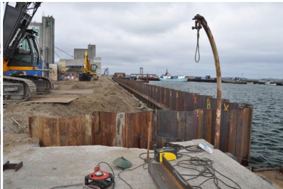
Sheet pile mounting completed.
